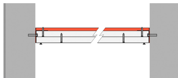
Assembly without support structure
