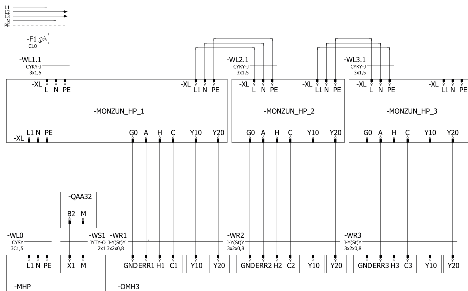
Fig. 4: Connection diagram of MONZUN-HP aggregates with the OMH3 control box
