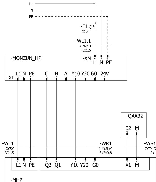
Fig. 2: Connection diagram of the MONZUN-HP unit with the MHP control box
