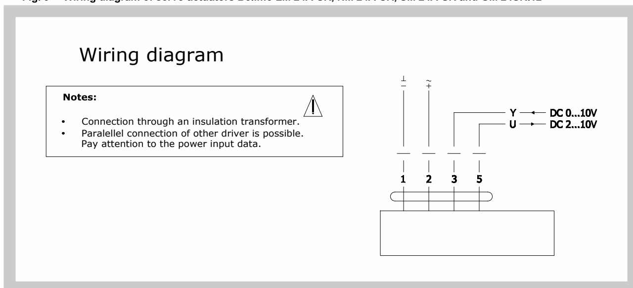
Fig. 9 Wiring diagram of servo actuators Belimo LM 24A-SR, NM 24A-SR, SM 24A-SR and GM 24SR.12
