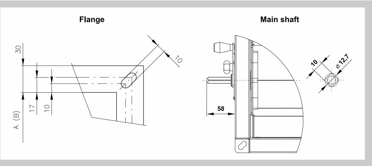
Fig. 6 Connection dimensions
