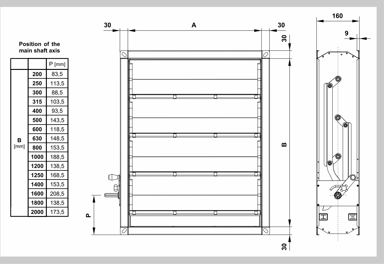
Fig. 5 Damper dimensions
