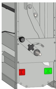
Fig. 3 Damper with manual control including handle and locking nut
