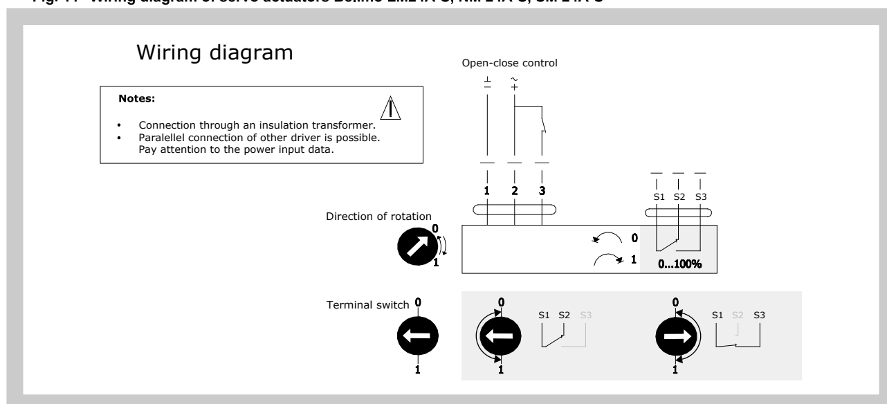
Fig. 11 Wiring diagram of servo actuators Belimo LM24A-S, NM 24A-S, SM 24A-S
