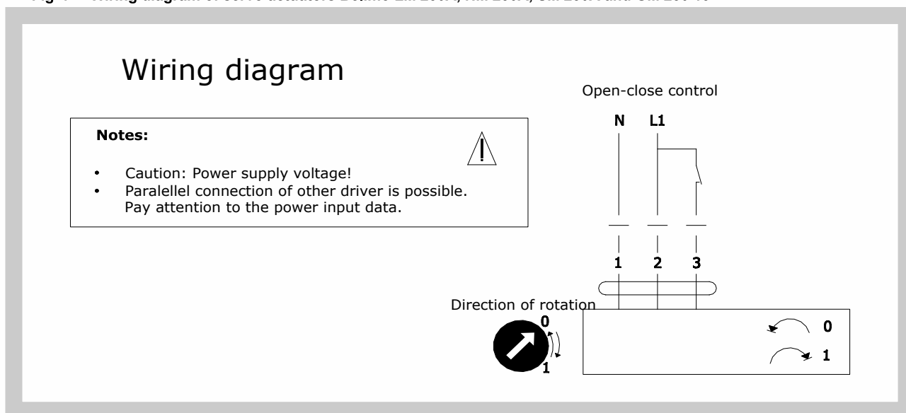
Fig. 8 Wiring diagram of servo actuators Belimo LM 24A, NM 24A, SM 24A and GM 24.13
