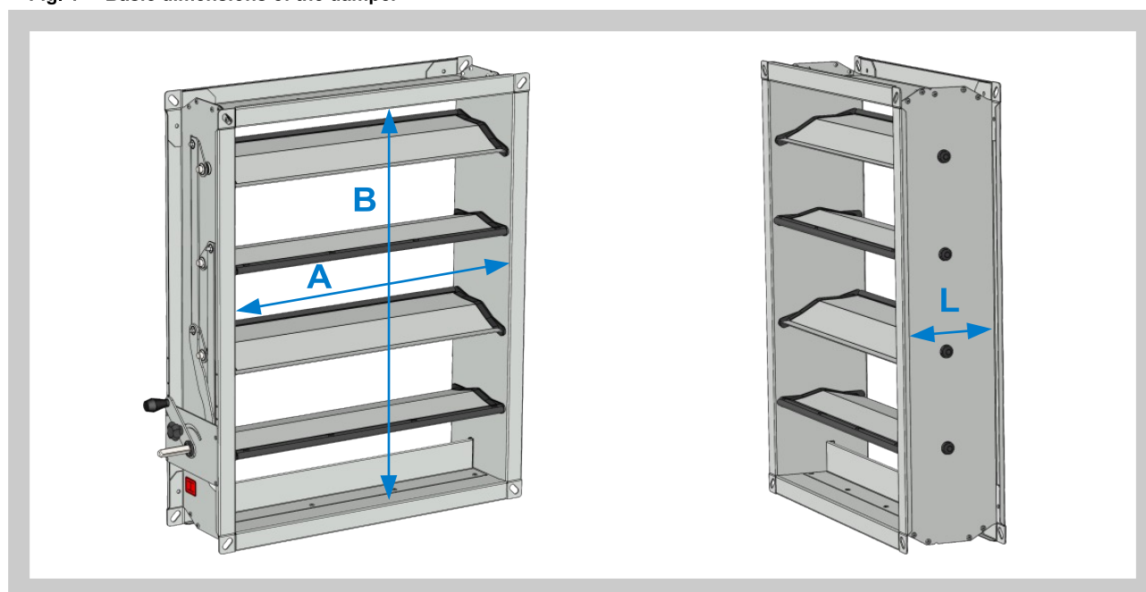
Fig. 1 Basic dimensions of the damper
