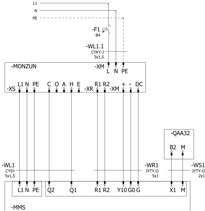
Fig. 2: Connection diagram of the MONZUN heater with the MMS control box
