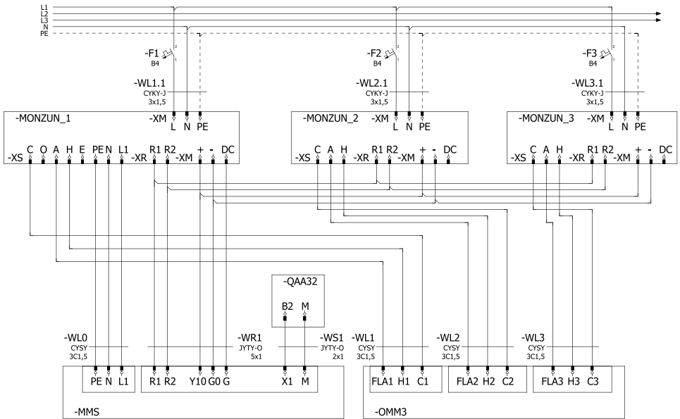
Fig. 4: Connection diagram of MONZUN aggregates with the OMM3 control box
